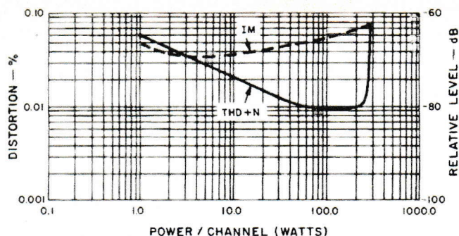
Fig. 7—THD and noise vs. power output.
